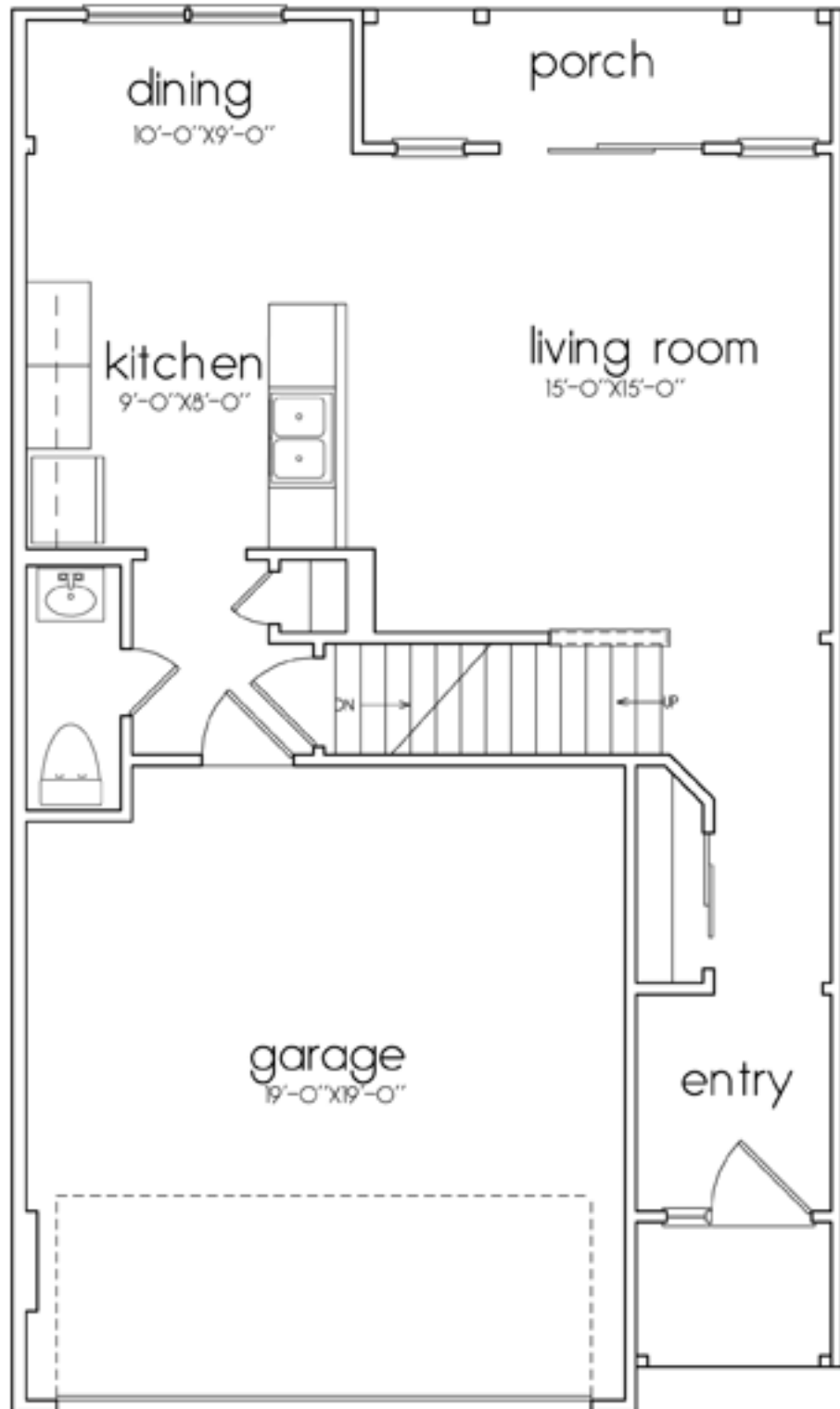
1st floor plan 2-story unit
